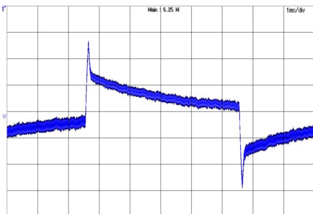
Figure 5: Output voltage response to step-change in load current (50%-75%-50% of full load; di/dt = 0.1A/\mu s ). Trace: Vout, 100mV/div; Time: 1ms/div
