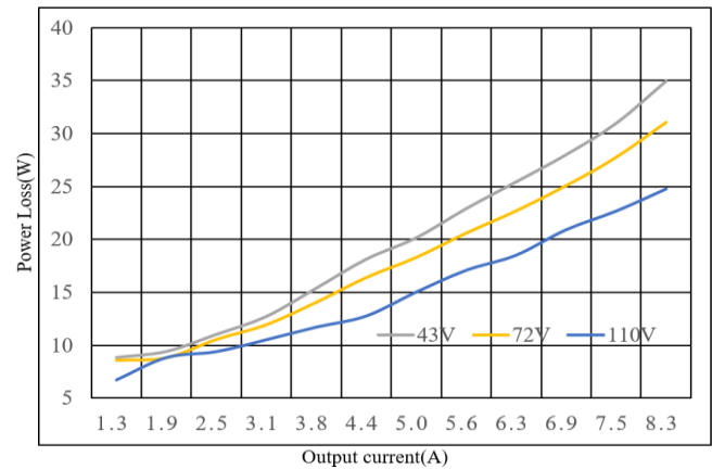
Figure 20: Power loss vs. load current at 25°C.
