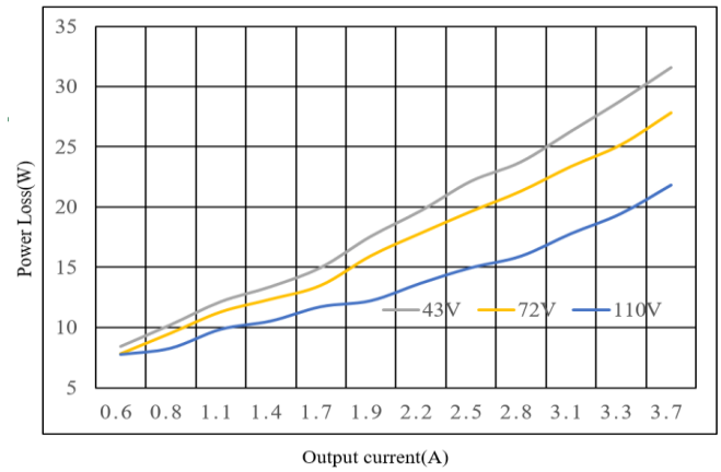
Figure 26: Power loss vs. load current at 25°C.
