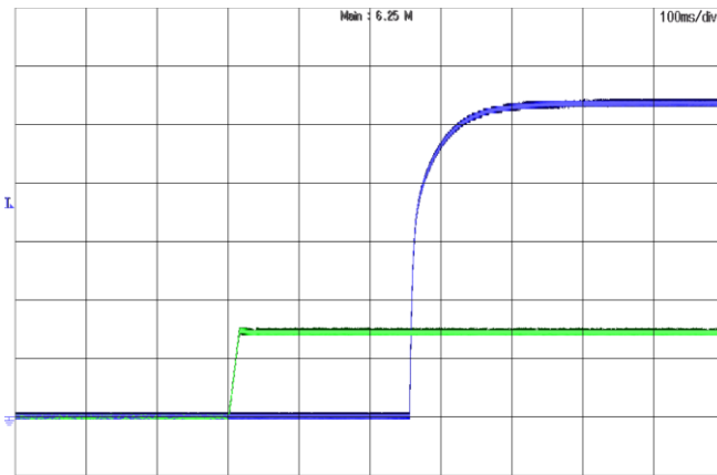
Figure 27: Turn-on transient at full load current (100ms/div). Top Trace: Vout, 10V/div; Bottom Trace: Vin, 50V/div
