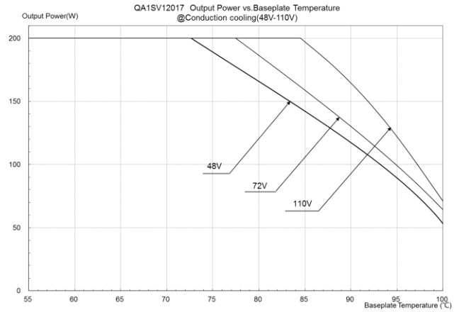
Figure 35: Output power vs. base plate temperature @ V_{in}=48\sim 110V V_{out}=12V or 15V
