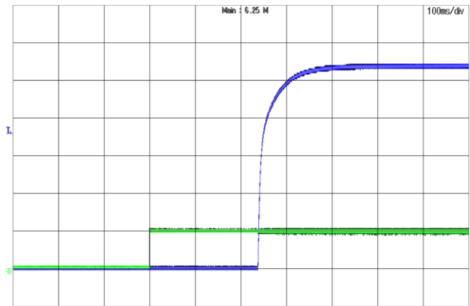
Figure 28: Turn-on transient at full load current (100ms/div). Top Trace: Vout, 10V/div; Bottom Trace: ON/OFF, 5V/div
