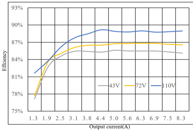
Figure 19: Efficiency vs. load current at 25°C.
