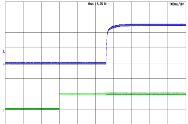
Figure 10: Turn-on transient at full load current (100ms/div). Top Trace: Vout, 5V/div; Bottom Trace: ON/OFF, 5V/div
