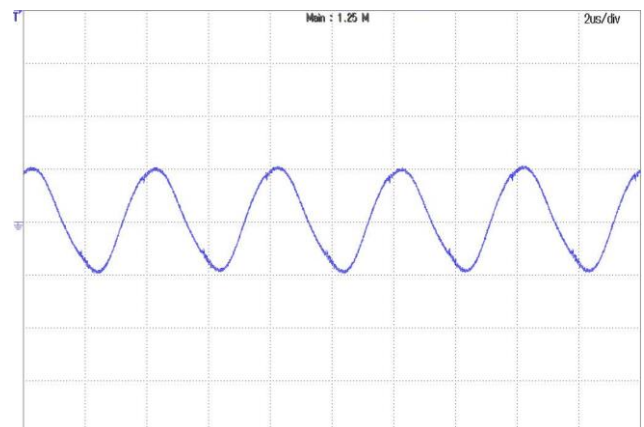
Figure 18: Output voltage ripple at Vin=110V and full load Trace: Vout, 100 mV/div, 2us/div; Bandwidth: 20 MHz.
