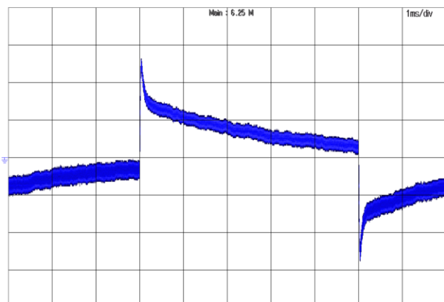
Figure 23: Output voltage response to step-change in load current (50%-75%-50% of full load; di/dt = 0.1A/\mu s ). Trace: Vout, 100mV/div; Time: 1ms/div
