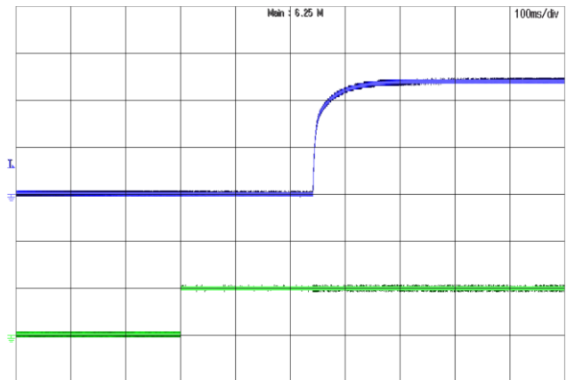
Figure 22: Turn-on transient at full load current (100ms/div). Top Trace: Vout, 2V/div; Bottom Trace: ON/OFF, 5V/div
