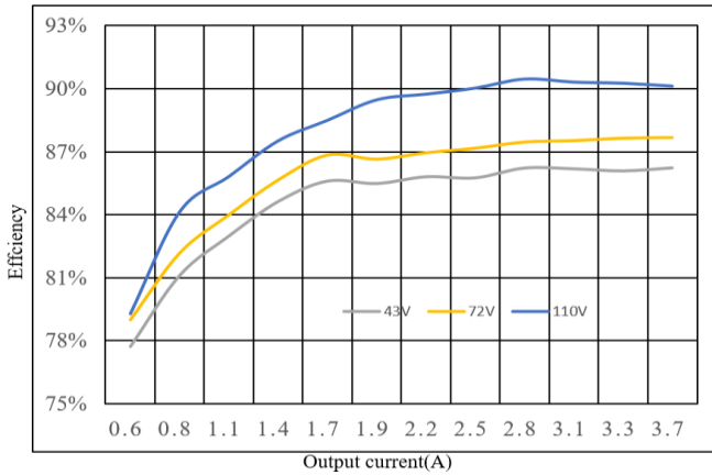
Figure 25: Efficiency vs. load current at 25°C.
