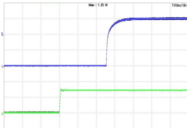
Figure 15: Turn-on transient at full load current (100ms/div). Top Trace: Vout, 5V/div; Bottom Trace: Vin, 75V/div
