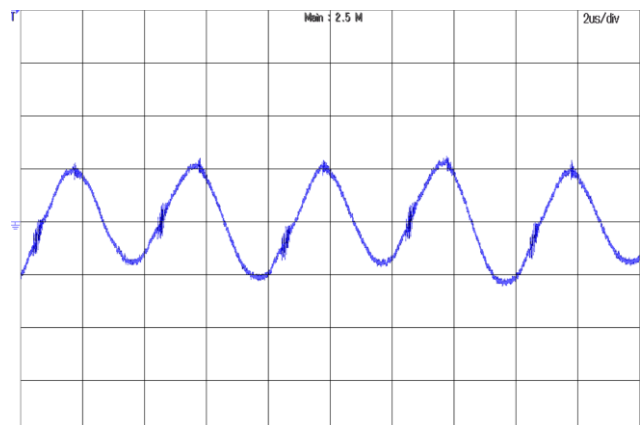
Figure 24: Output voltage ripple at V_{in}=110V and full load Trace: Vout, 20 mV/div, 2us/div; Bandwidth: 20 MHz.
