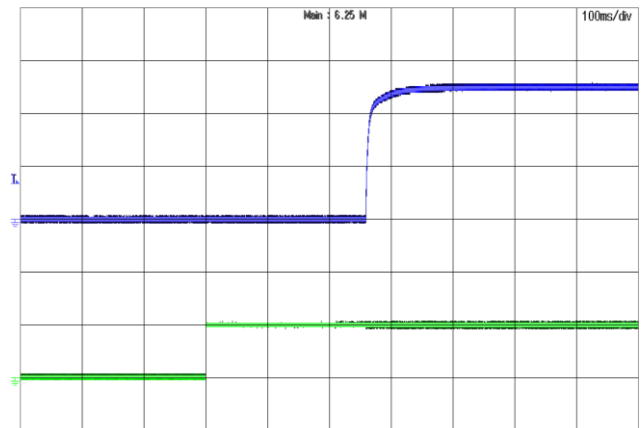
Figure 4: Turn-on transient at full load current (100ms/div). Top Trace: Vout, 2V/div; Bottom Trace: ON/OFF, 5V/div
