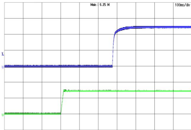
Figure 3: Turn-on transient at full load current (100ms/div). Top Trace: Vout, 2V/div; Bottom Trace: Vin, 75V/div
