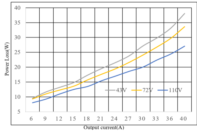
Figure 2: Power loss vs. load current at 25°C.
