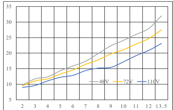
Figure 14: Power loss vs. load current at 25°C.
