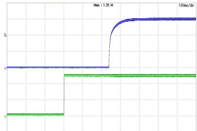
Figure 16: Turn-on transient at full load current (100ms/div). Top Trace: Vout, 5V/div; Bottom Trace: ON/OFF, 5V/div
