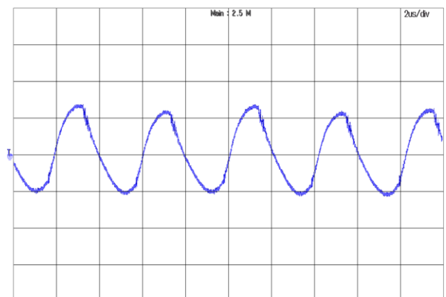
Figure 6: Output voltage ripple at Vin=110V and full load Trace: Vout, 20 mV/div, 2us/div; Bandwidth: 20 MHz.
