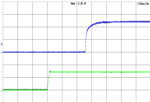
Figure 21: Turn-on transient at full load current (100ms/div). Top Trace: Vout, 2V/div; Bottom Trace: Vin, 75V/div
