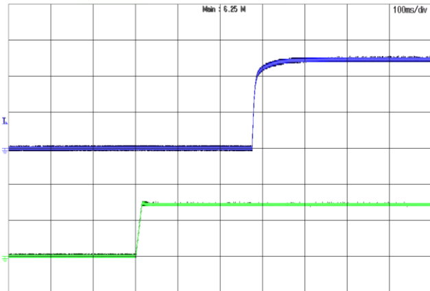
Figure 9: Turn-on transient at full load current (100ms/div). Top Trace: Vout, 5V/div; Bottom Trace: Vin, 75V/div
