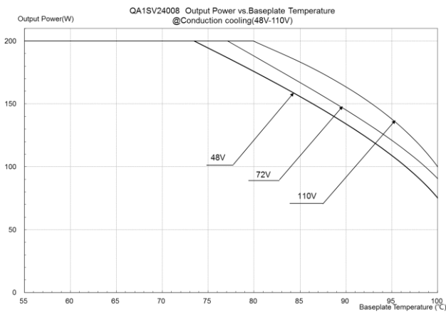
Figure 36: Output power vs. base plate temperature @ V_{in}=48\sim 110V V_{out}=24V
