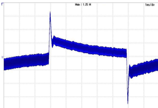
Figure 17: Output voltage response to step-change in load current (50%-75%-50% of full load; di/dt = 0.1A/\mu s ). Trace: Vout, 200mV/div; Time: 1ms/div
