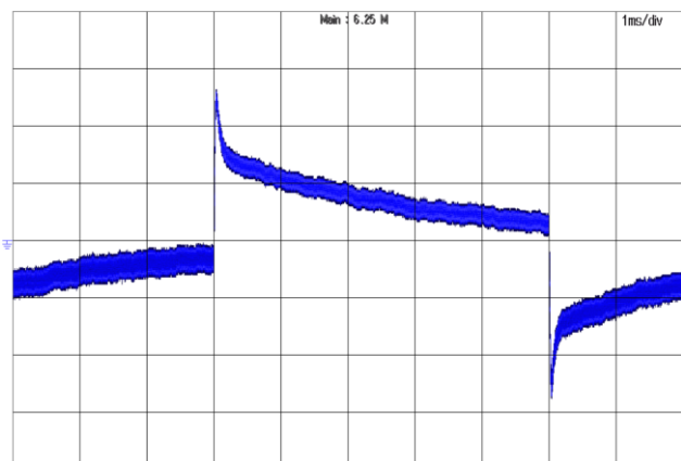
Figure 11: Output voltage response to step-change in load current (50%-75%-50% of full load; di/dt = 0.1A/\mu s ). Trace: Vout, 500mV/div; Time: 1ms/div
