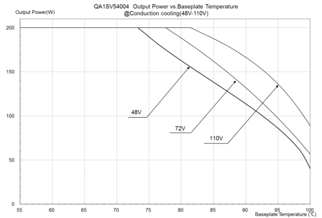
Figure 37: Output power vs. base plate temperature @ V_{in}=48\sim 110V V_{out}=54V
