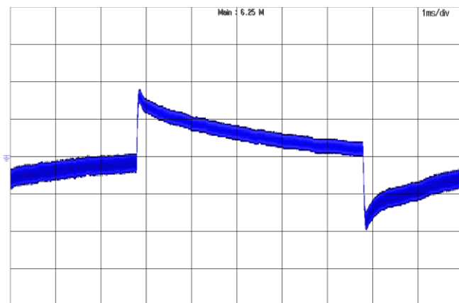
Figure 29: Output voltage response to step-change in load current (50%-75%-50% of full load; di/dt = 0.1A/\mu s ). Trace: Vout, 500mV/div; Time: 1ms/div
