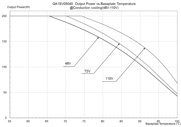
Figure 34: Output power vs. base plate temperature @ V_{in}=48\sim 110V V_{out}=5V
