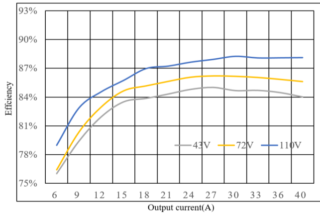
Figure 1: Efficiency vs. load current at 25°C.
