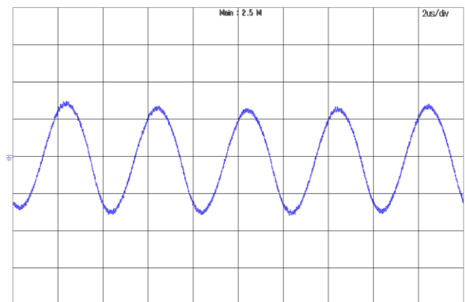
Figure 30: Output voltage ripple at V_{in}=110V and full load Trace: Vout, 100 mV/div, 2 \mu s /div; Bandwidth: 20 MHz.
