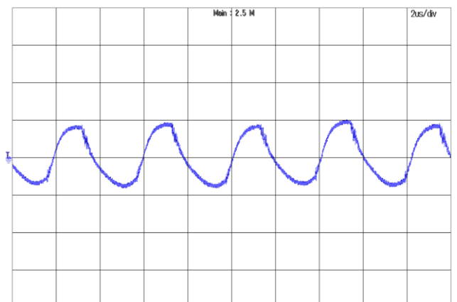
Figure 12: Output voltage ripple at V_{in}=110V and full load Trace: Vout, 100 mV/div, 2us/div; Bandwidth: 20 MHz.
