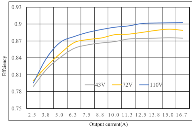
Figure 7: Efficiency vs. load current at 25°C.
